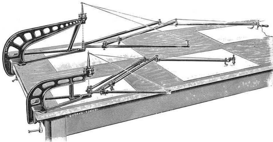
Pantograph extra large of 150 cm and Pantograph Type I 96 cm bars both with frame No 18 f. with suspendet foot.
