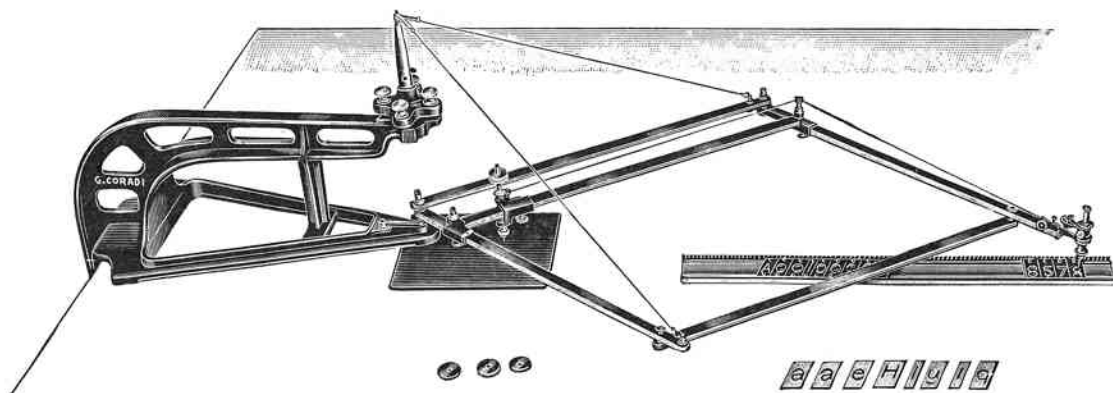
Pantograph arranged for engraving respectively for the reproduction of characters, chiffres for the nomenclature of maps etc. with special clamping device for the patterns.
