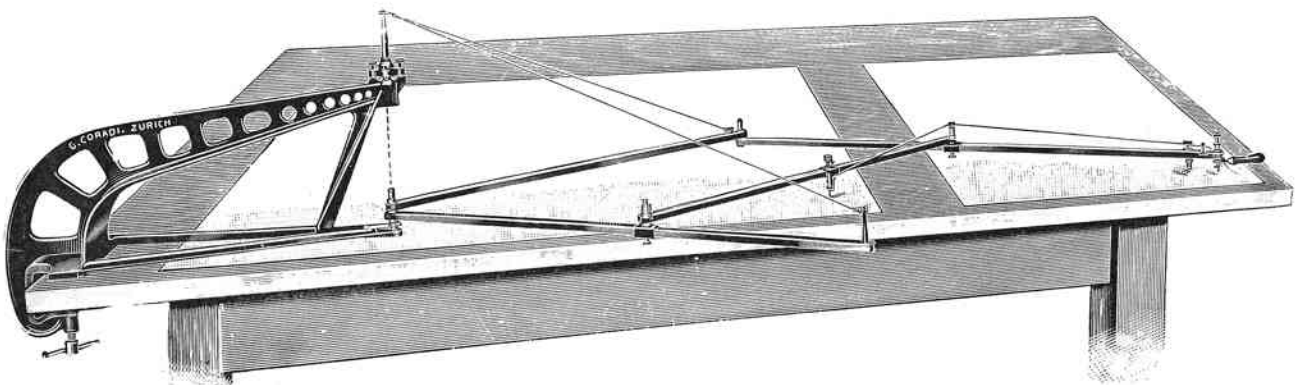
Pantograph extra large model length of the bars 150 cm
