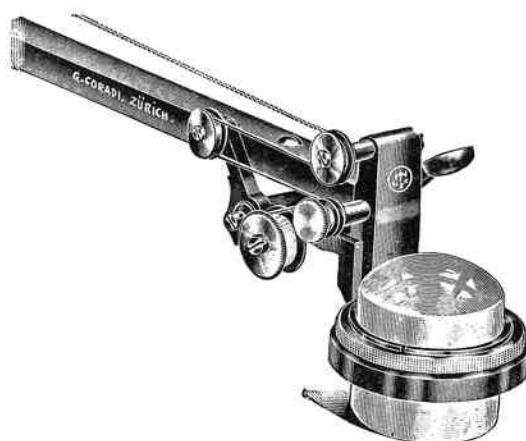
The new magnifying-glass-tracer.
