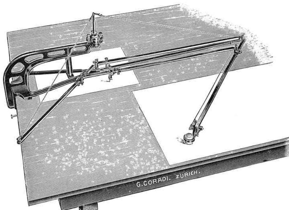
Pantograph with new magnifying-glass-tracer and new release arrangement and supplied with frame No. 18 f.
